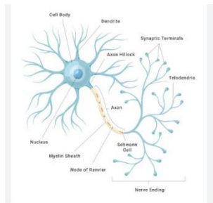
Figure 1.1.6: Neuron Structure [11]
