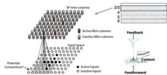
Figure 1.1.9: Representation of spatial pooler [12]
