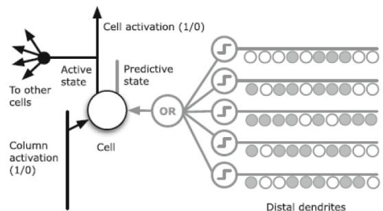
Figure 1.1.3: Distal Dendrite Segment at the Cellular Level [13]
