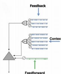
Figure 1.1.2: Proximal Dendrite Representation [9]
